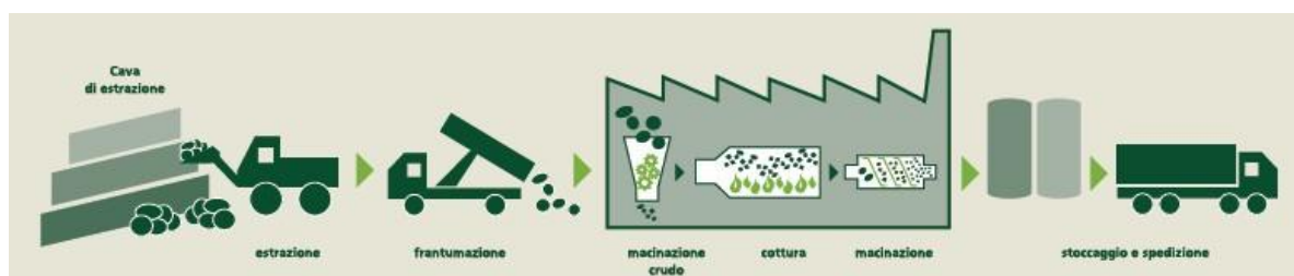
Figure 3 - Cement production process
